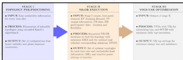
Figure 29: Stage-wise approach for integrated VVO, NR, and DR in active unbalanced EDNs
