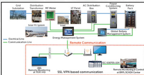
Figure 61: Schematic of Category-C Pilot by TERI/BRPL
