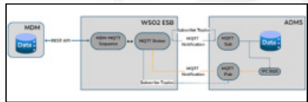
Figure 34: MDM – WSO2 ESB – ADMS in Kanpur field pilots
