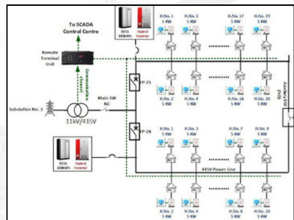
Figure 52: Communication Architecture and HMI interface
