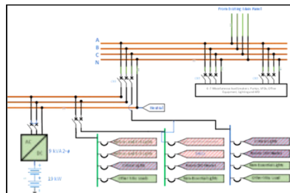
Figure 63: WSU distribution system with BESS near McCluskey Services building
