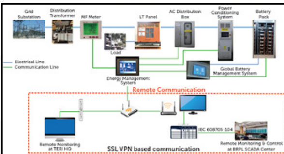
Figure 58: Schematic of Category-A Pilot by TERI/BRPL
