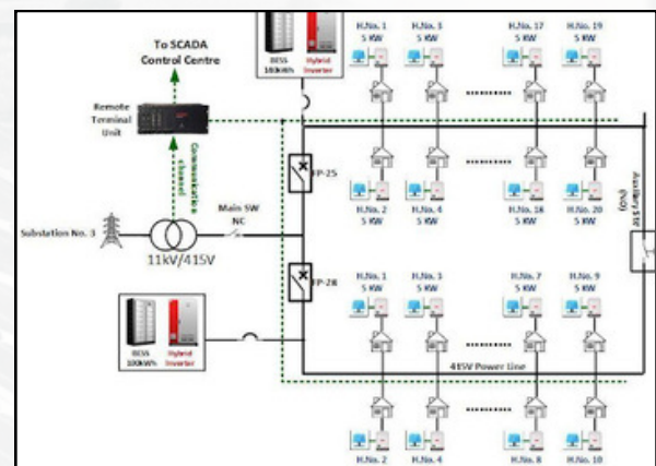
Figure 50: Schematic of Semi-urban field pilot
