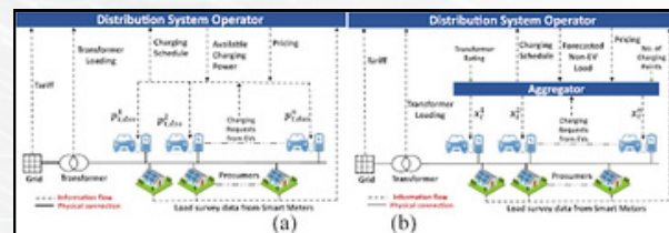
Figure 31: Proposed (a) centralized, and (b) decentralized EV pricing strategies
