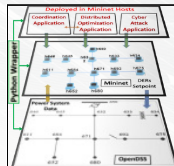
Figure 76: OpenDSS and Mininet based CPS co-simulation testbed
