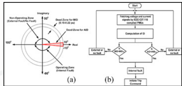
Figure 22: (a) Magnitude phase plane of ID, (b) Flowchart of proposed ID-based protection and fault detection scheme
