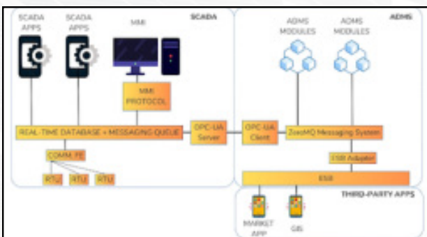
Figure 33: Developed ADMS architecture
