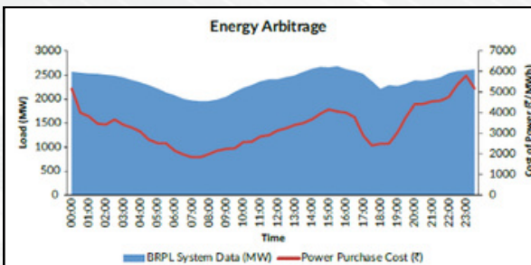
Figure 59: Energy Arbitrage in Category-A Pilot
