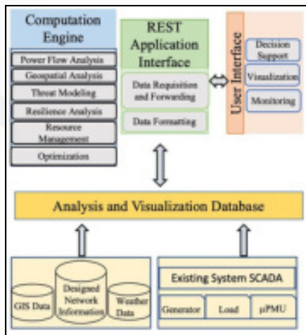
Figure 91: Overview of the RT-RMS Dataflow Architecture
