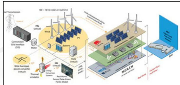
Figure 81: NREL testbed
