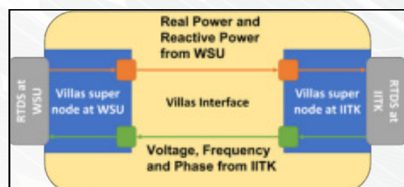
Figure 93: Villas interface for federated co-simulation
