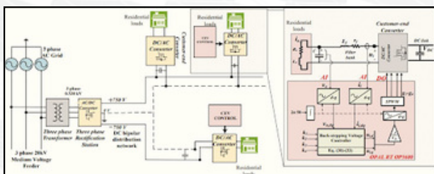
Figure 17: Field test environment for LV DC distribution implementation
