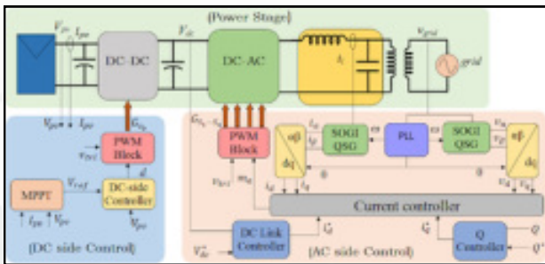
Figure 15: Complete control architecture of a solar PV based DER connected to the main AC grid.
