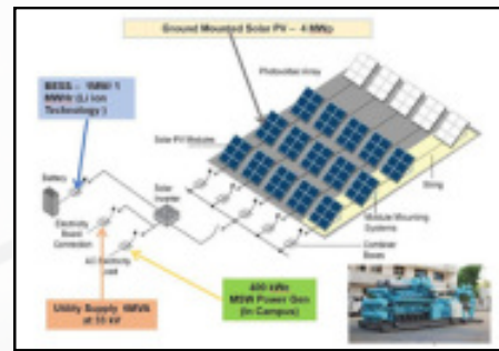
Figure 53: Schematic of NETRA Semi-urban field Pilot
