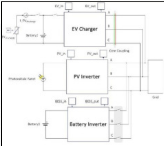
Figure 83: Schematic of the n-grid model implemented on Typhoon-HIL
