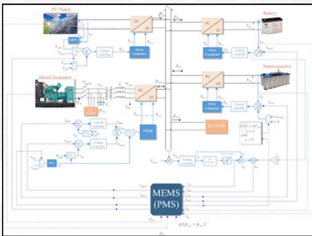
Figure 19: DC microgrid architecture with control mechanism under islanded mode.
