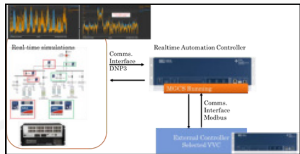
Figure 65: VVC Testing with AVISTA field model using HIL
