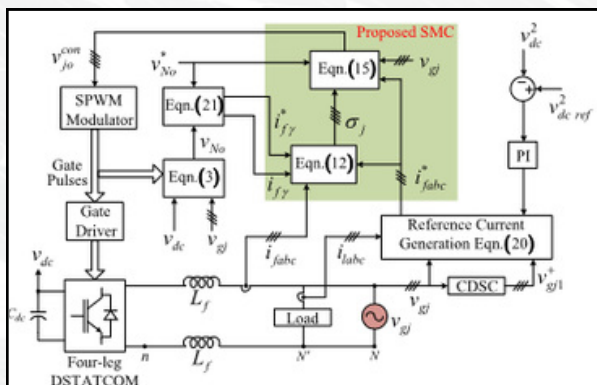
Figure 13: Block diagram of the SMC control scheme as primary controller
