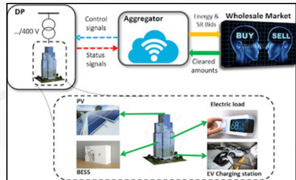
Figure 25: Nanogrid based aggregator framework
