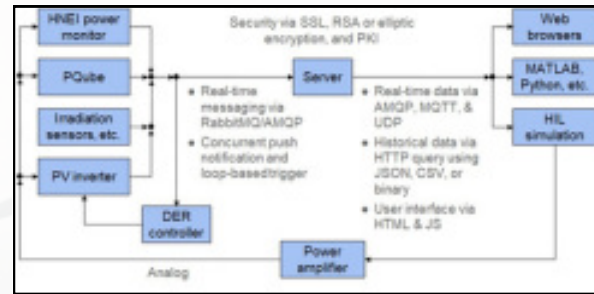
Figure 79: Communication architecture
