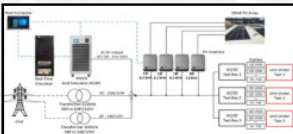
Figure 77: HIL testbed block diagram
