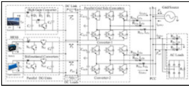
Figure 14: Proposed hybrid microgrid structure
