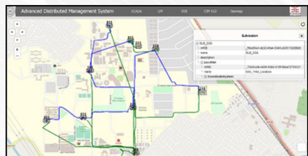
Figure 35: GIS mapping of IIT Kanpur distribution network in the developed ADMS HMI
