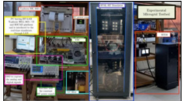
Figure 72: Testbed for real-time validation of an Anti-Islanding Protection Scheme of IBRs
