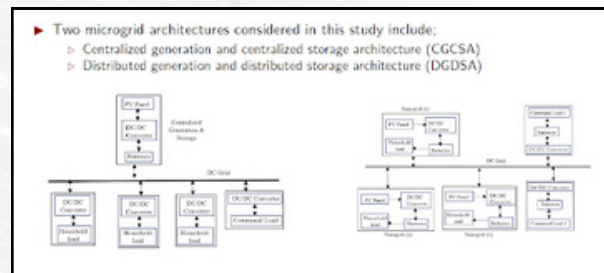
Figure 18: Two different architectures of rural DC grids: 1) Centralized generation centralized storage (Left side), 4) Distributed generation distributed storage (Right side).
