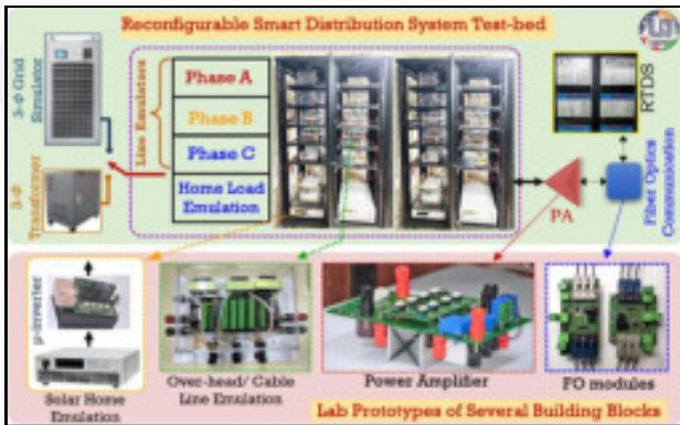
Figure 71: Overview of the LV distribution system test bed
