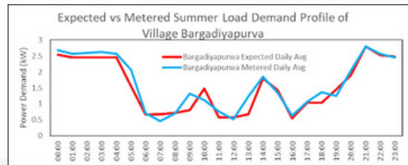
Figure 42: Expected vs Metered Load Demand Profile in Rural Pilot
