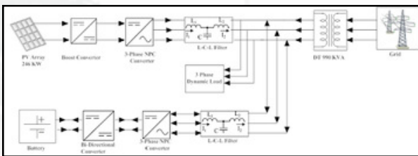
Figure 6: System level modelling of BESS for WSU Urban distribution system
