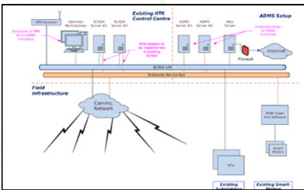
Figure 32: Schematic of existing SCADA and Newly Developed ADMS at IIT Kanpur
