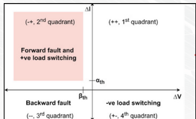
Figure 23: Scheme of proposed \Delta V - \Delta I plane-based fault detection & classification in LV DC microgrids
