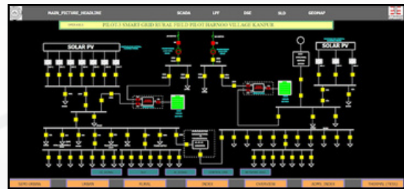
Figure 57: MEMS screen of ADMS application for Rural field Pilot
